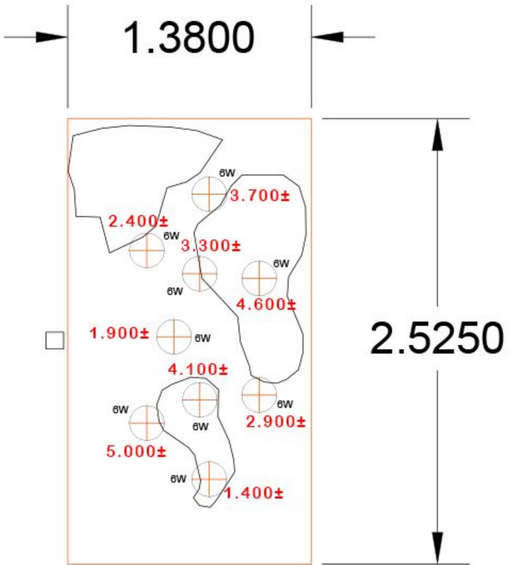
INCANDESCENT LIGHT LAYOUT
